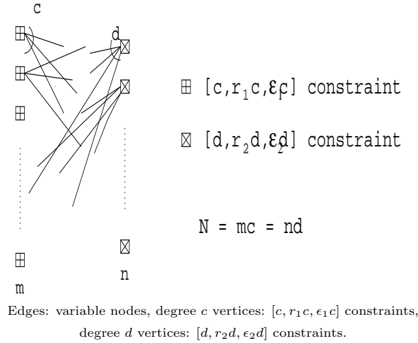
FIGURE 6. Expander code: Case D.
