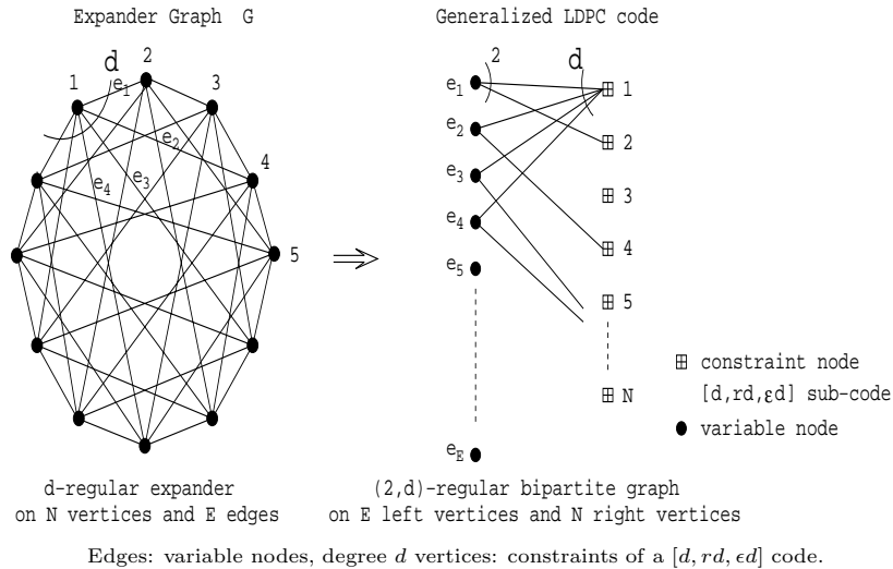
FIGURE 5. Expander code: Case C.
